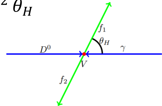
Figure 20: Definition of the helicity angle.
