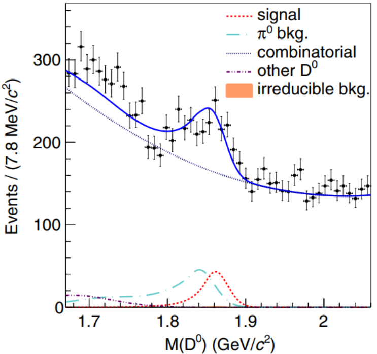
Shape of Signal: Crystal-Ball Irreducible background were said before
