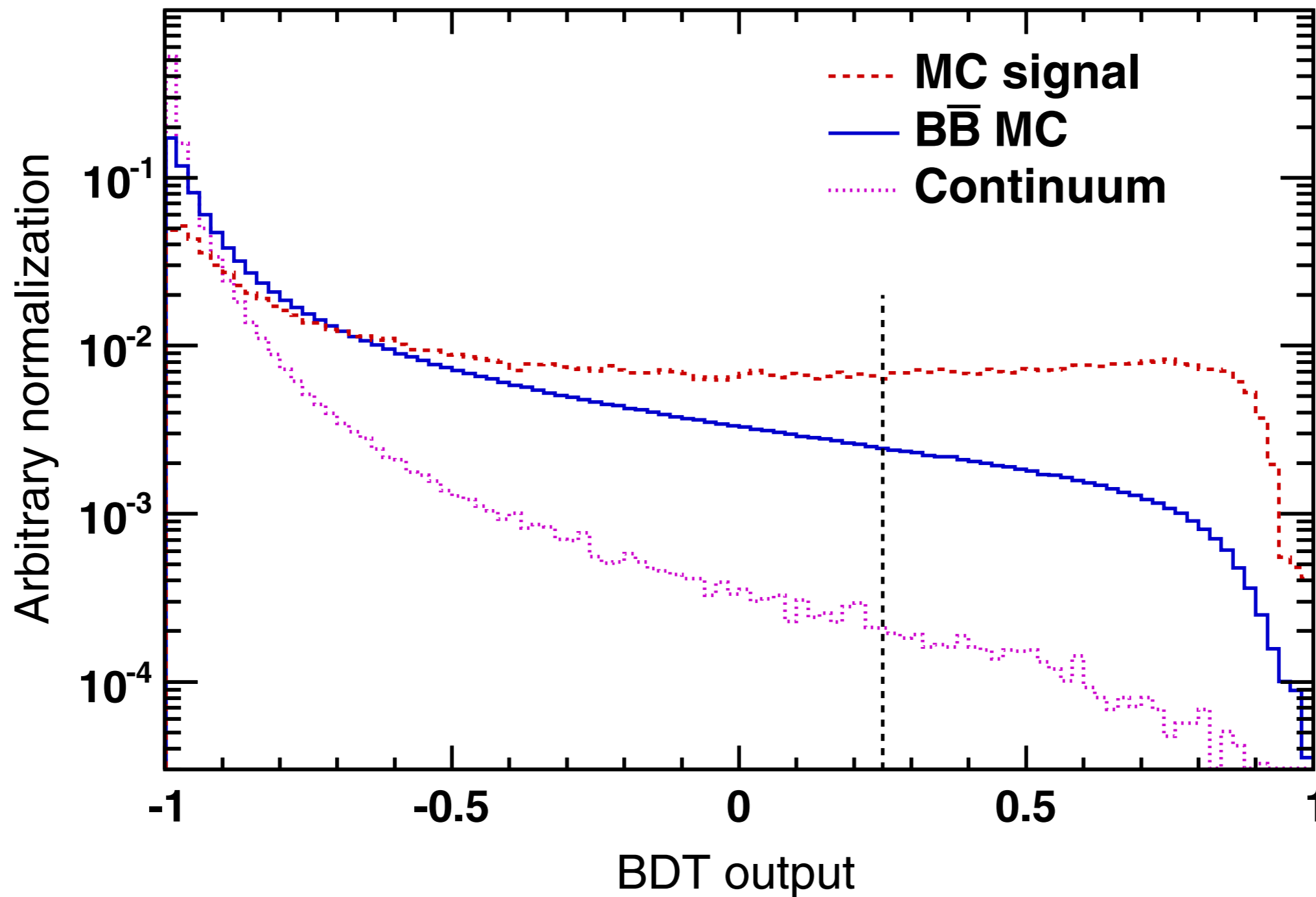
FIG. 2 (color online). Output of the BDT. The continuum distribution corresponds to off-resonance data. The vertical line denotes the minimum requirement on this variable.
