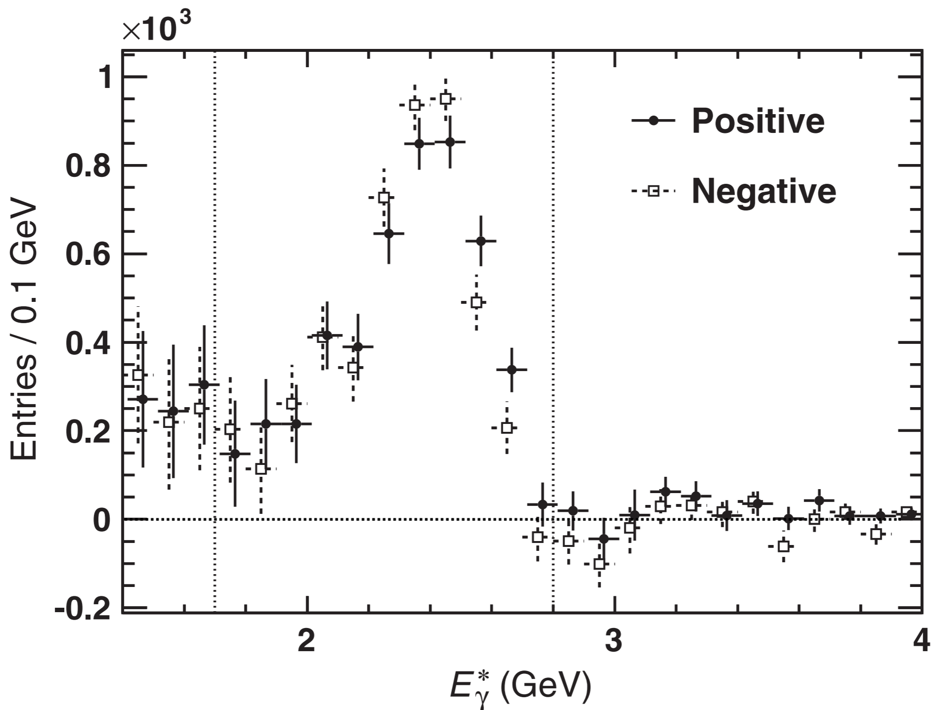
FIG. 3. The photon energy spectrum in the c.m. system after subtracting all the background, with vertical dashed lines showing the signal region. The positive tagged events are shown as circles and the negative as squares. Statistical and systematic uncertainties are included.
